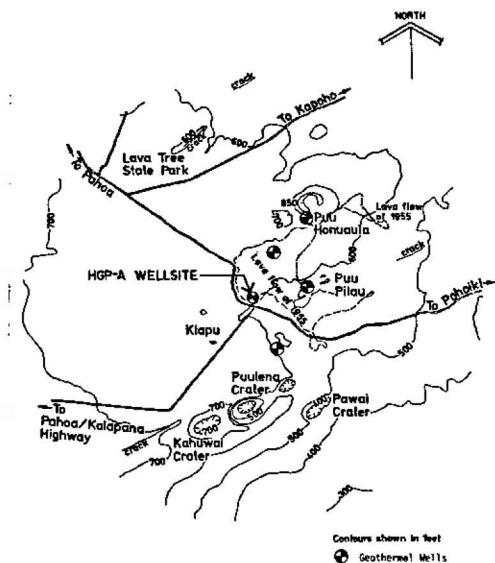
Figure 2. Geothermal Locations
