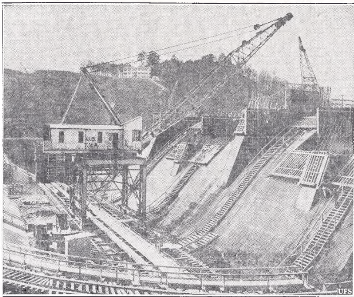
SPILLWAY —Taking form on Tennessee river in East Tennessee is spillway of TVA's Watts Bar dam. Closing of dam gates for first impounding of water is scheduled for December of this year. Completed dam will be 97 feet high; 2,965 feet long, with reservoir of 41,600 acres extending 72 miles upstream. It's for electrical power.
