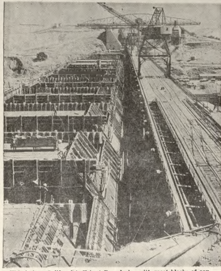
This is how California's Friant Dam looks, with most blocks of concrete built up to level of 220-foot high construction trestle. They must be built up another 100 feet, as indicated by completed section on Fresno County abutment at far end of trestle.
