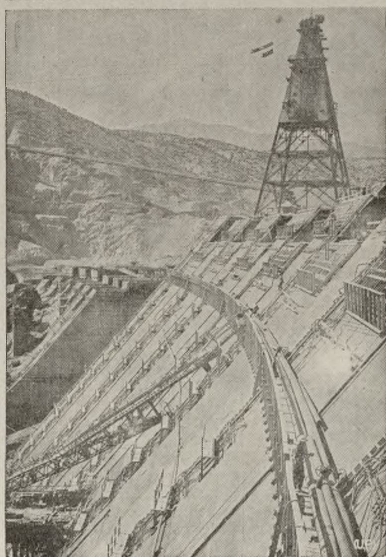
This interesting photo shows sloping, downstream face of big Shasta—a face that's changing constantly as engineers push the mighty, multiple-purpose barrier across California's Sacramento River. Note workers on temporary catwalks. Cableway head tower in background.
