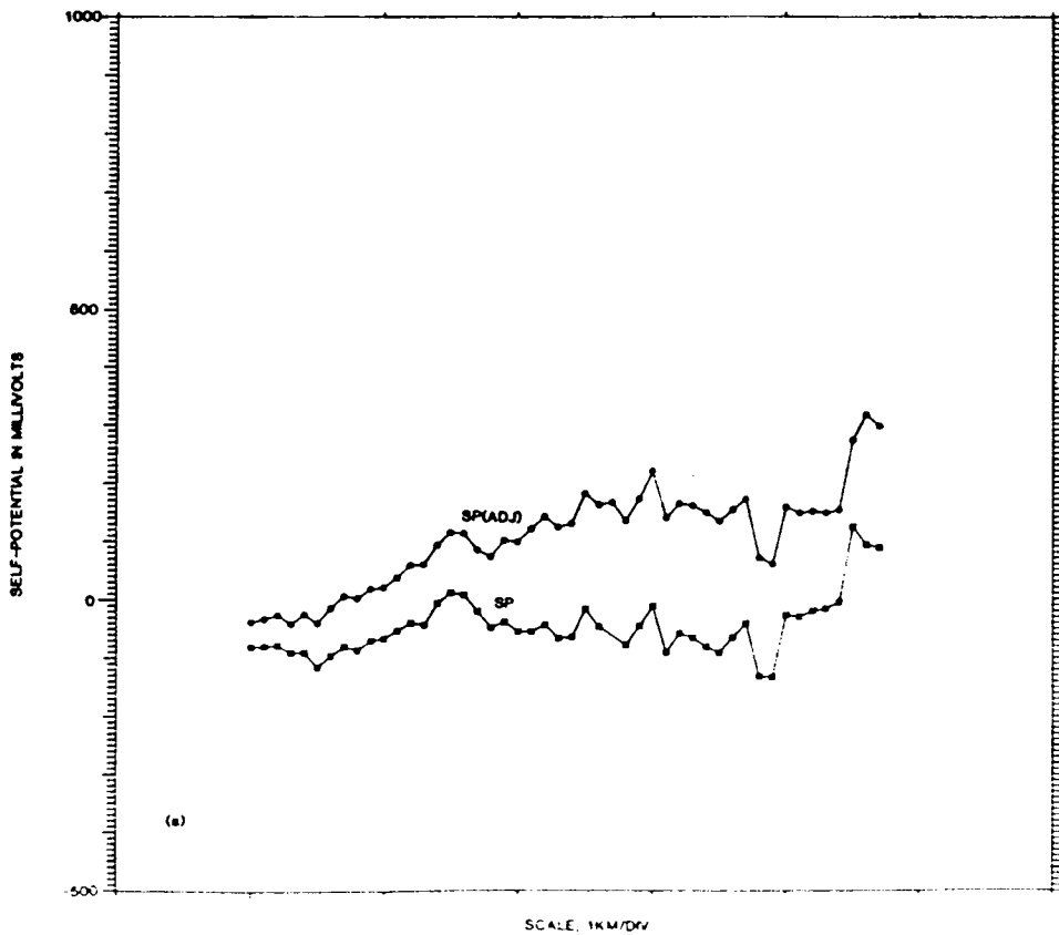
Figure 5. Profiles B-B' (5a) and C-C' (5b), southeast flank of Hualalai. Adjusted profiles are corrected by 1.57 mv/m relative to the Waha hole reference.
