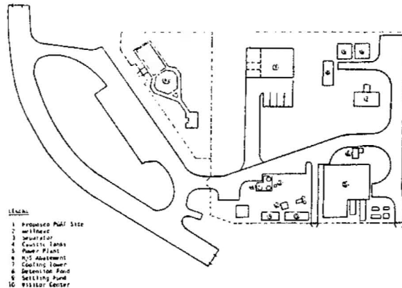
Figure 2. HGP-A Wellsite
